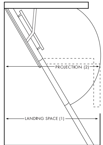
FIGURE 1 - WOOD STAIRWAYS
